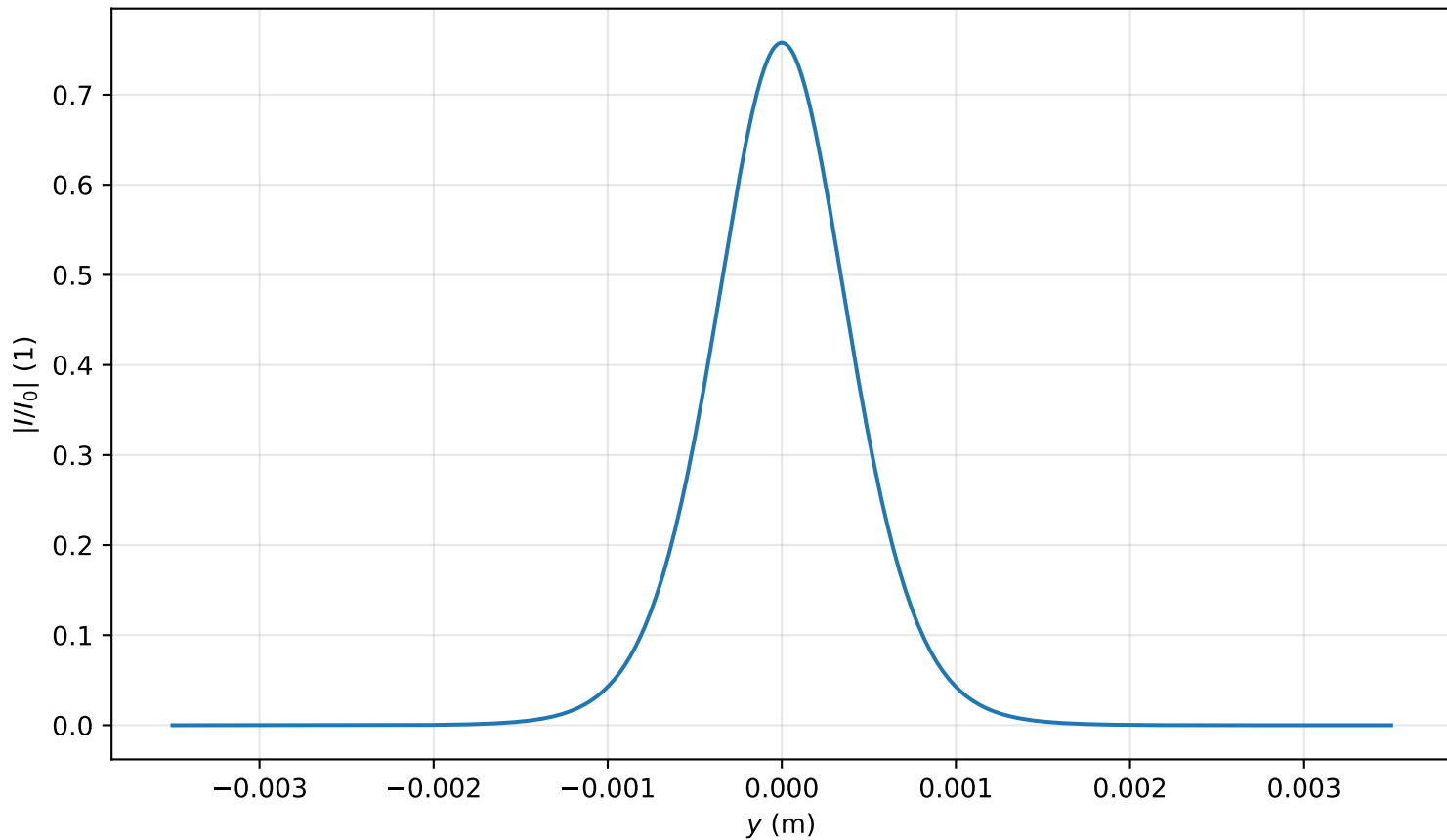
Intensity profile I(x=0, y, z=2.229)/I_0 , P_{in}=0.5P_{cr} , artificial time
